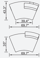
Arm C Module (Right)
